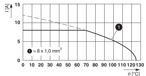
I = current strength, \vartheta = ambient temperature, 8 x 8 A
